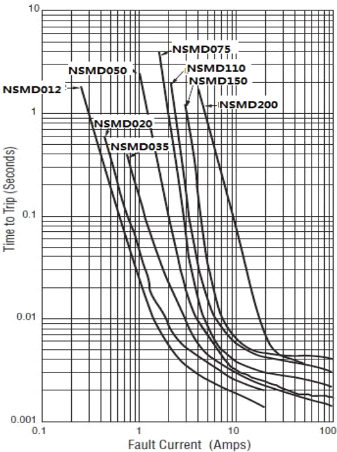
Typical time to trip at 25℃ (25℃下的动作保护时间曲线表):
