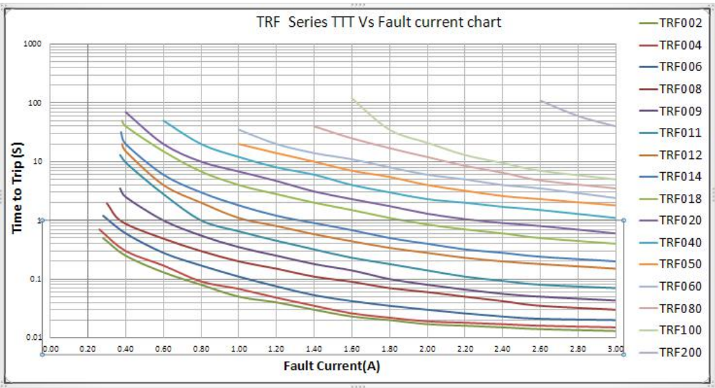
Typical time to trip at 25℃（25℃下的动作保护时间曲线表）:
